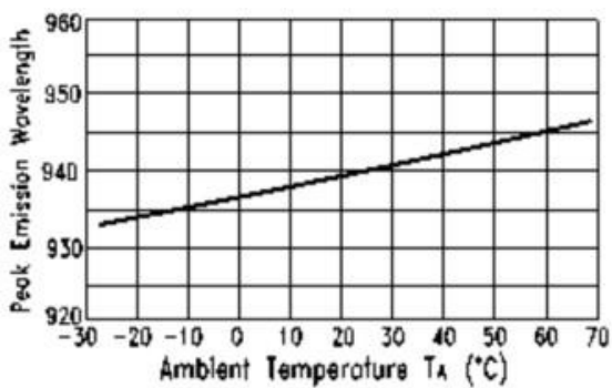
Fig.5 Peak Emission Wavelength vs. Ambient Temperature
