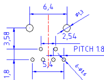
MOUNTING FOOTPRINT
